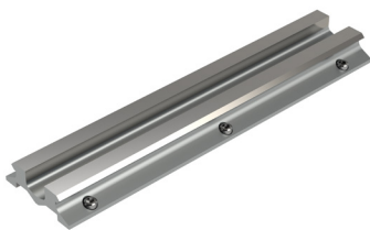
Track plate assembly consisting of two or more lengths of induction hardened steel track mounted to an anodized aluminum substrate
